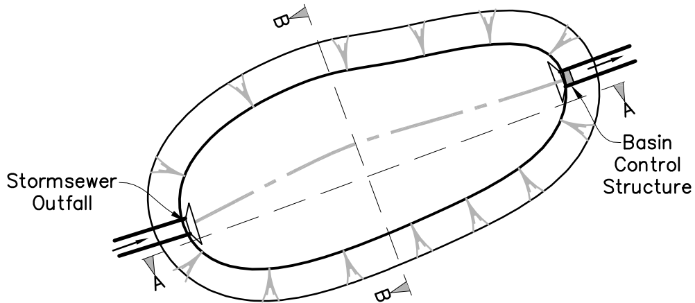
Typical Dry Detention Basin – Plan View
