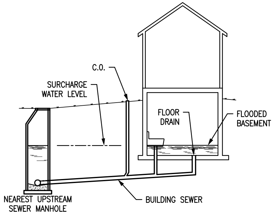
UNACCEPTABLE GRAVITY CONNECTION
