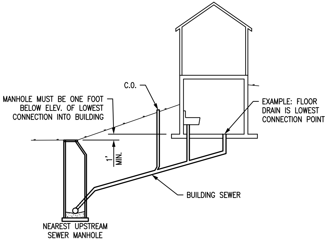
ACCEPTABLE GRAVITY CONNECTION
