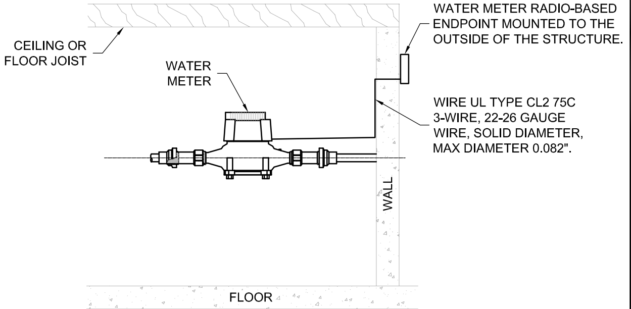
INTERIOR SECTION
