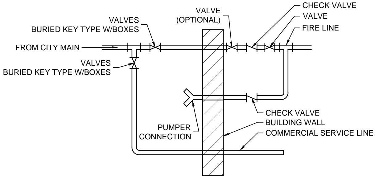
CHECK VALVE IN BUILDING
