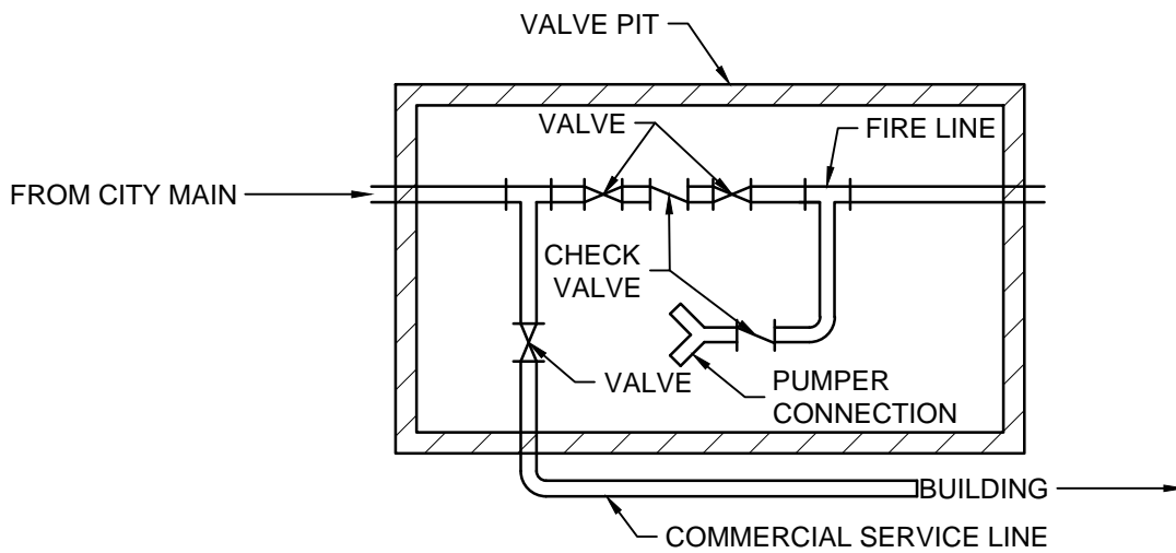
CHECK VALVE IN PIT
