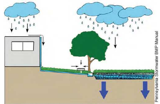
DIRECT CONNECTION OF A ROOF INTO A SUBSURFACE INFILTRATION BED
