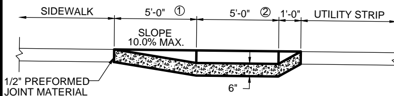
CURB ELEVATION
