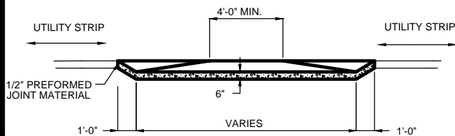
CURB ELEVATION
