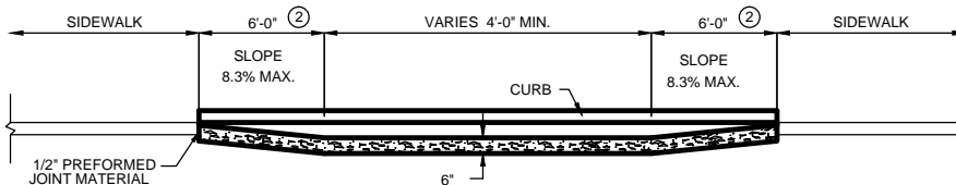
CURB ELEVATION
